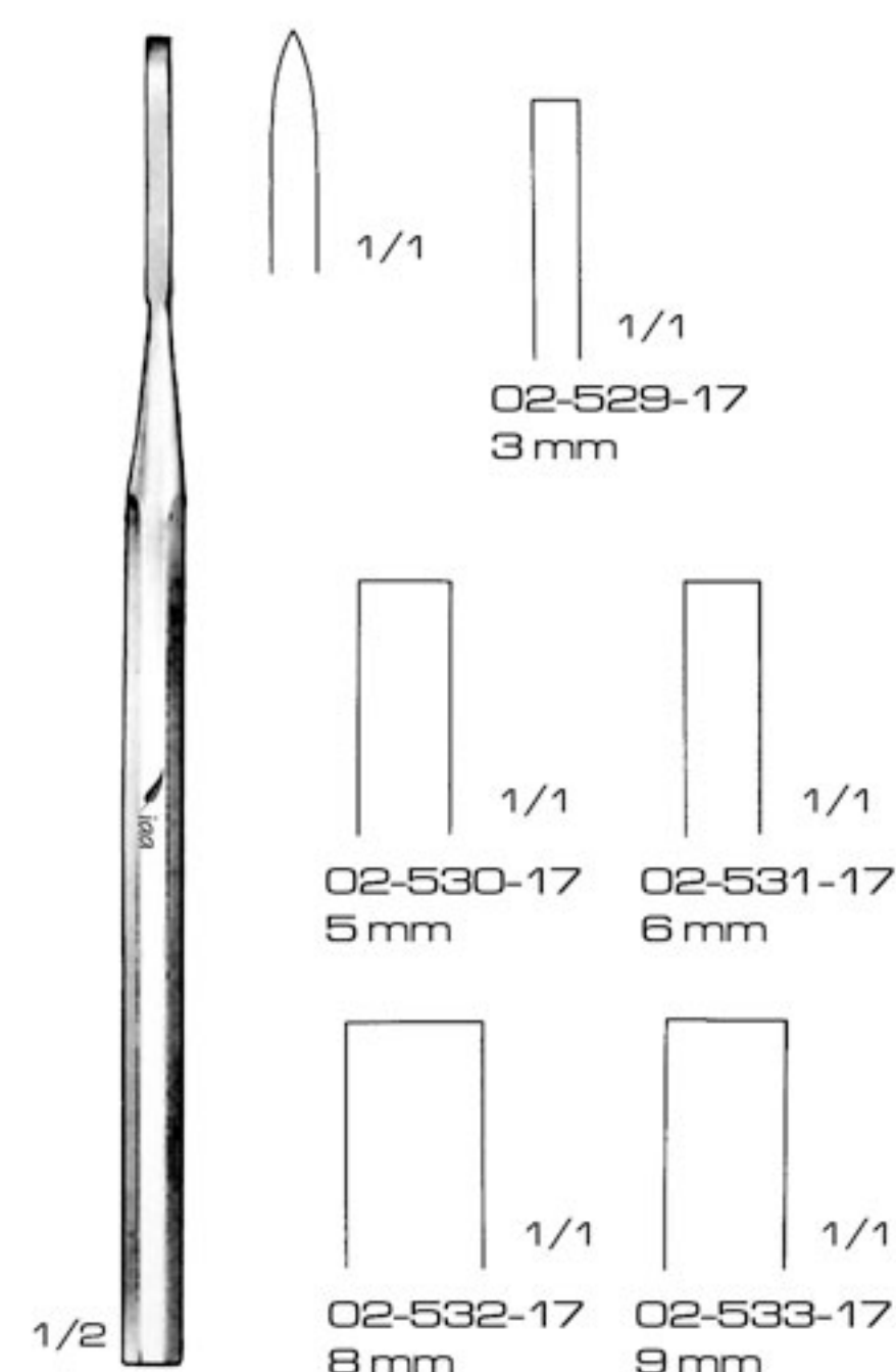
Hoke 02-529-17 To 02-533-17 17 cm / 6 3/4"
