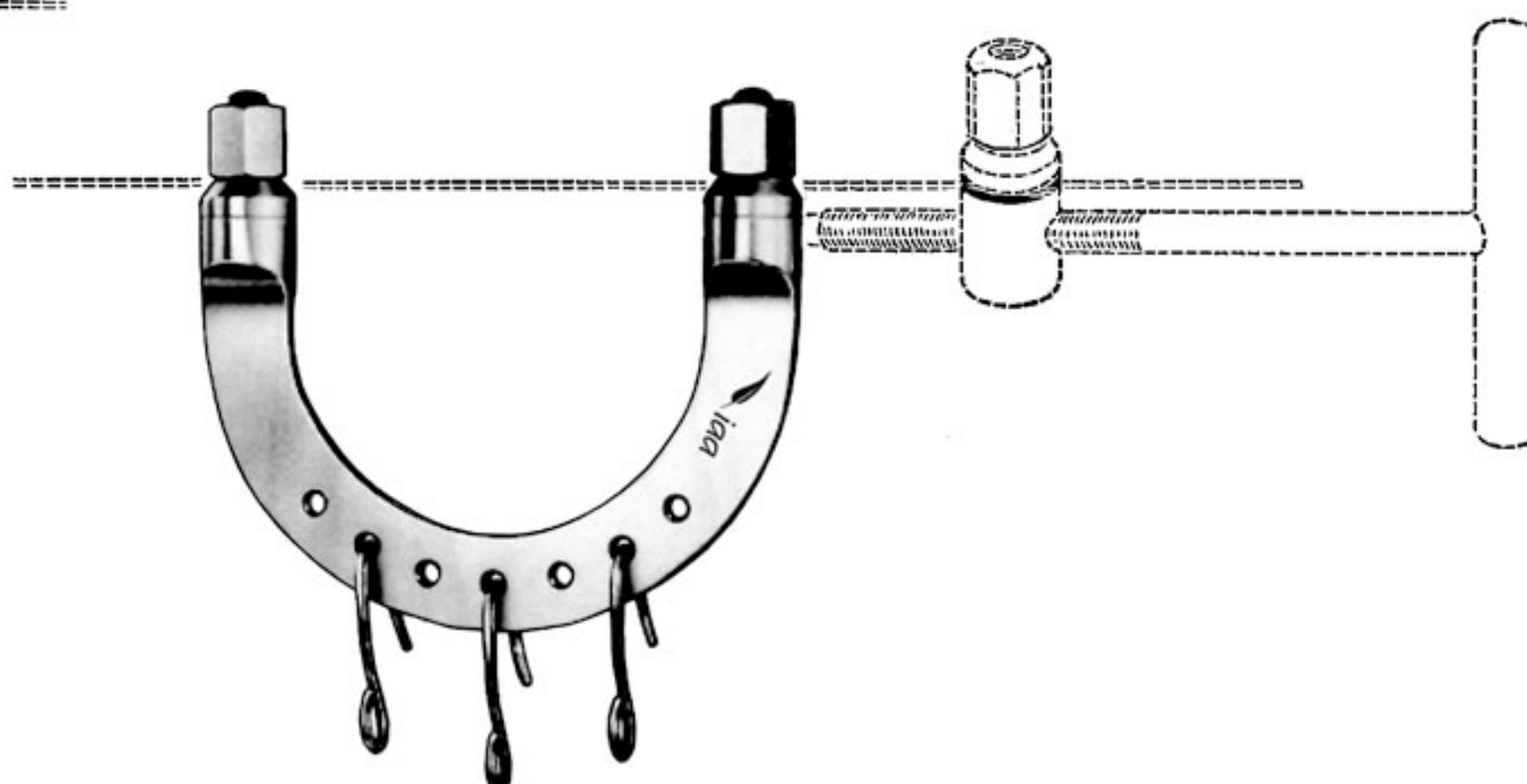
Kirschner 02-406-00 9.5 x 7 cm / 3 3 / 4 x 2 3 / 4 " 02-407-00 10.5 x 10.5 cm / 4 1 / 4 x 4 1 / 4 " 02-408-00 12 x 12 cm / 4 3 / 4 x 4 3 / 4 " 02-409-00 15 x 15 cm / 6 x 6" 02-410-00 20 x 15 cm / 8 x 6" With 3 traction pins
